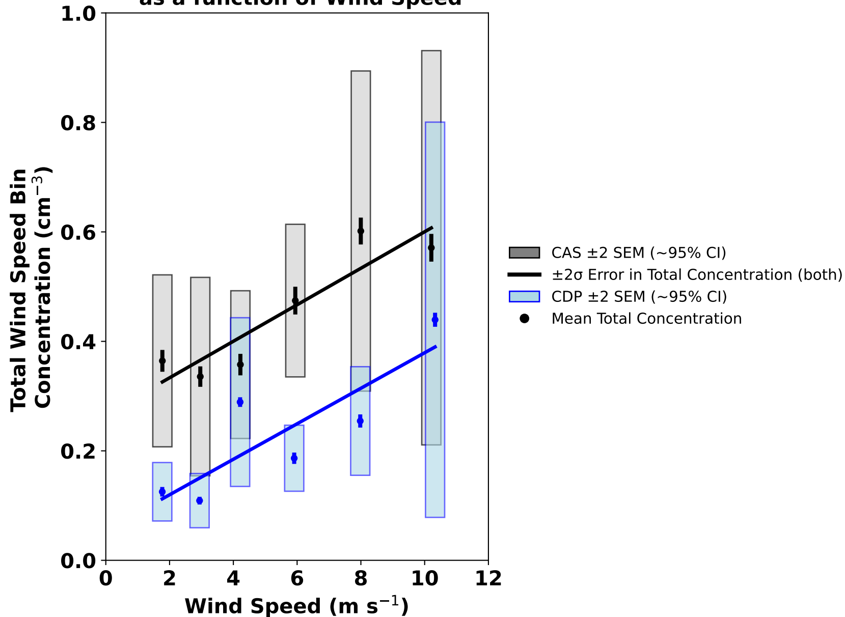
Binned GCCN Concentration as a function of Wind Speed
